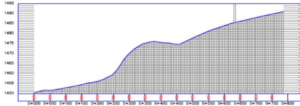
Rising Main PROFILE
