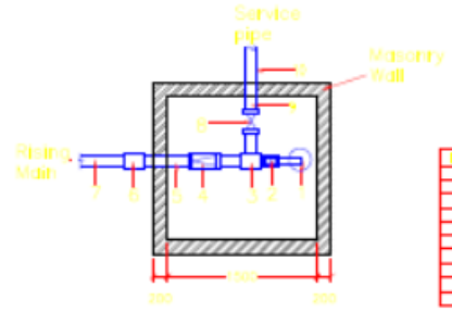
BORRHOLE CHAMBER PLAN
